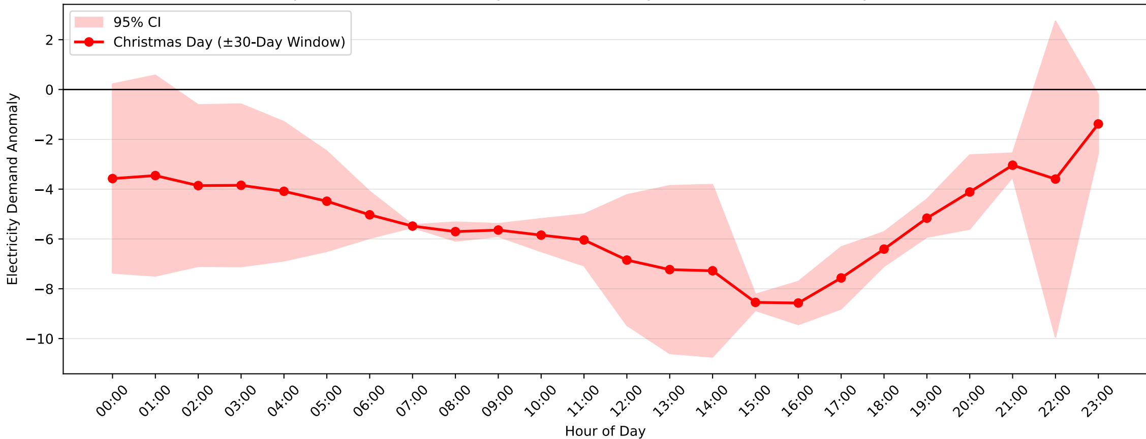
Campsie Demand Anomaly: Christmas Day (2009-2010, \pm 30 -Day Window)
