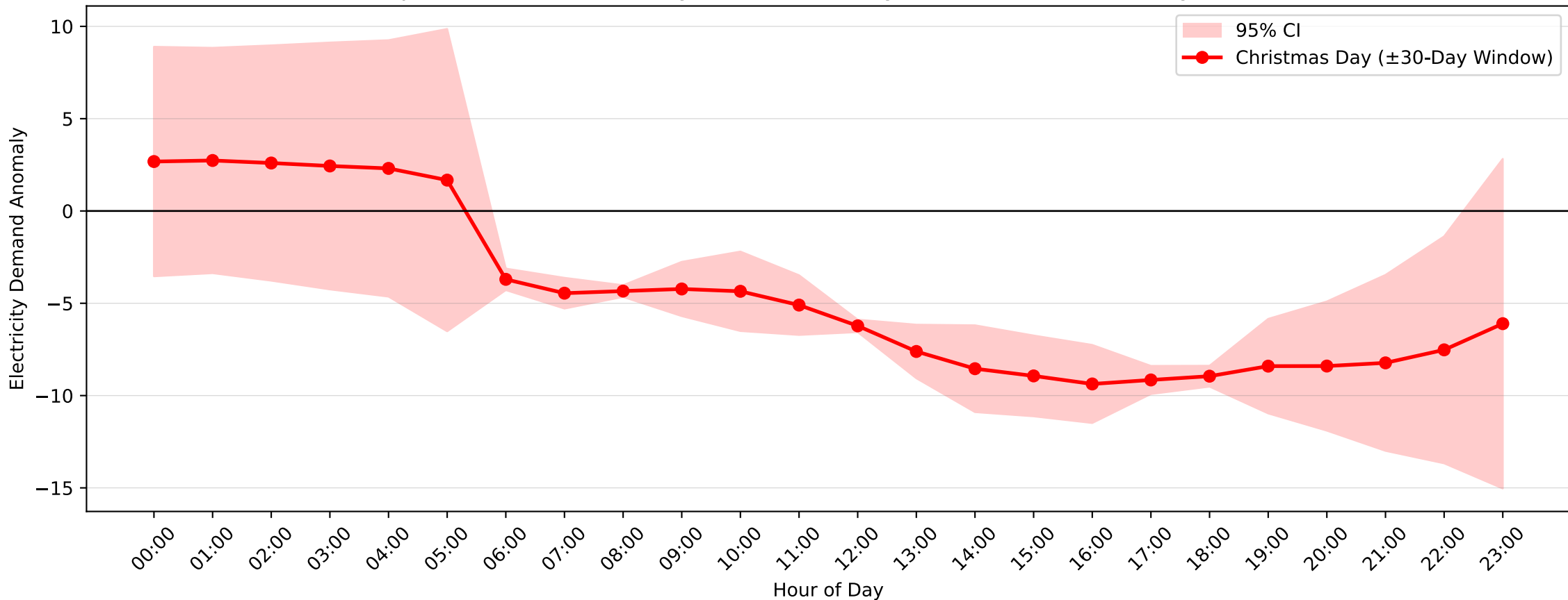
Campsie Demand Anomaly: Christmas Day (2013-2014, \pm 30 -Day Window)
